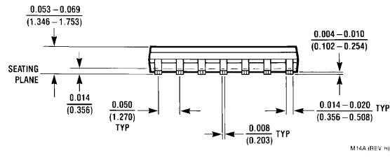
14-Lead Small Outline Molded Package (M) Order Number DM7404M Package Number M14A
